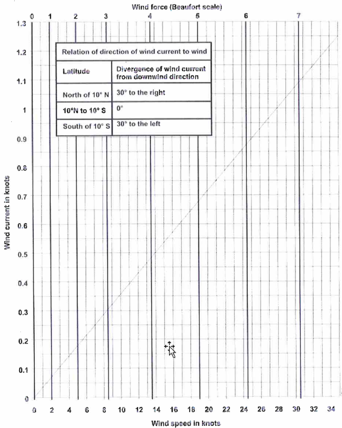
Figure D-5:1 Local Wind Current Graph
